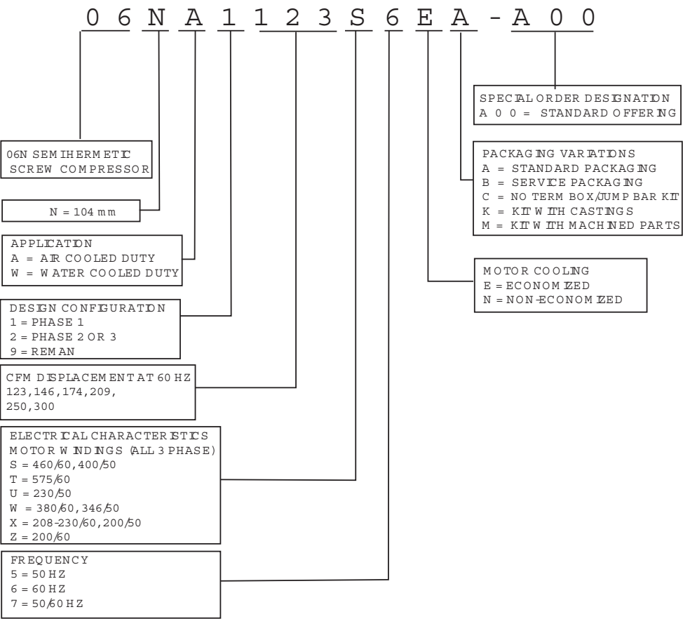
06N SCREW COMPRESSOR SIGNIFCANCE CHART
